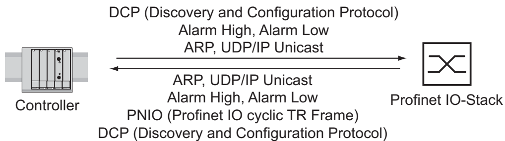
Figure 6: Communication between the Controller and the Switch
