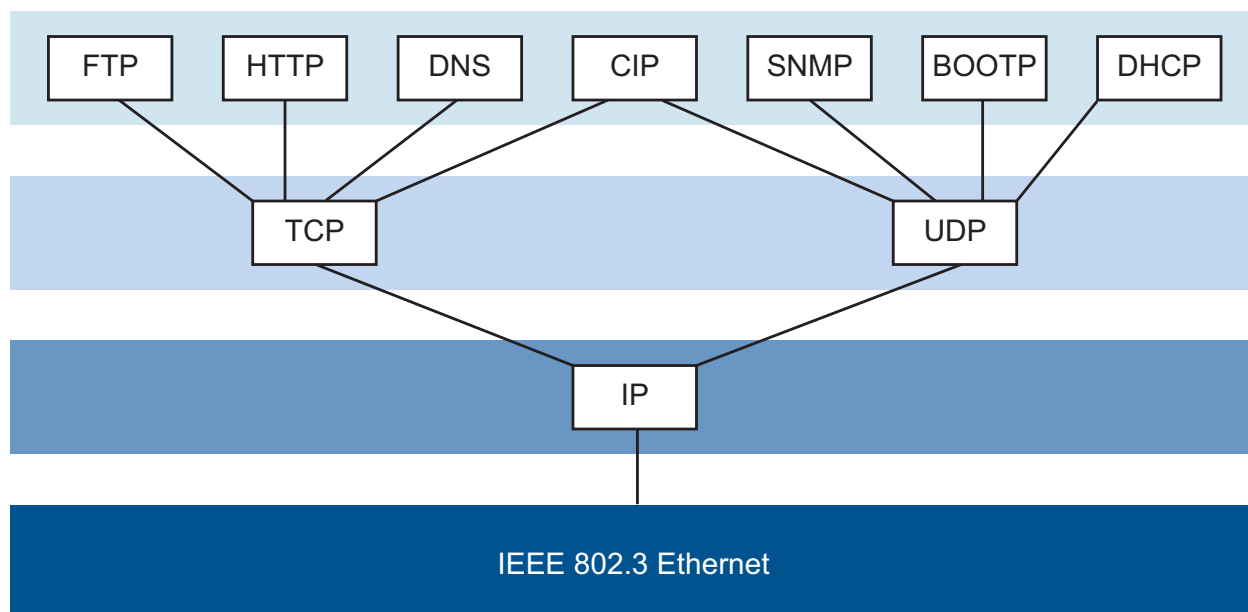
Figure 3: EtherNet/IP (CIP) in the ISO/OSI reference model
