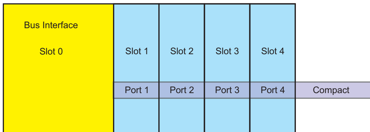
Figure 7: Compact Switch
