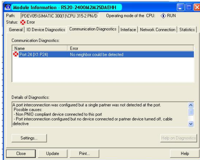
Figure 23: Diagnosis messages for the communication between the Switches and IO devices
